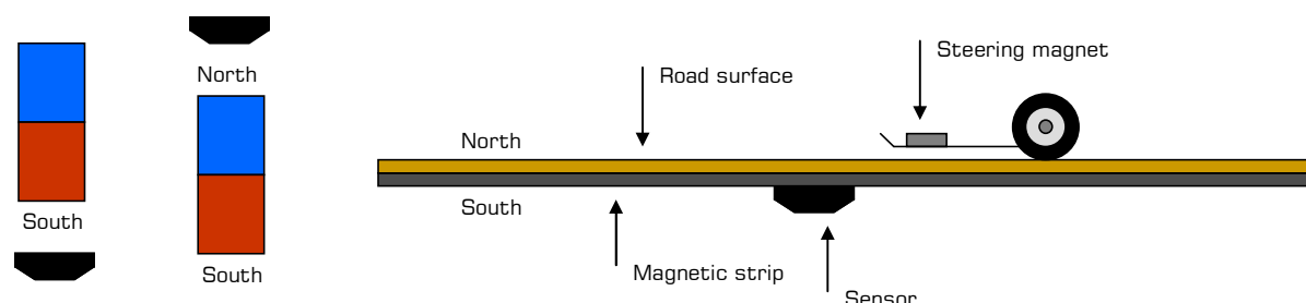
Figure 4: Orientation magnetism
