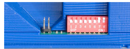
Fig24 : TM44 DIP switches
