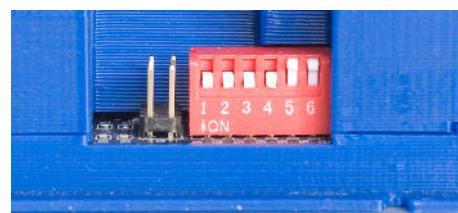
Fig 25: OC32/NG Dipswitches
