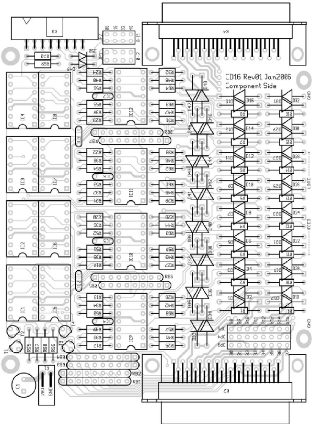
Fig 14: CD16 layout
